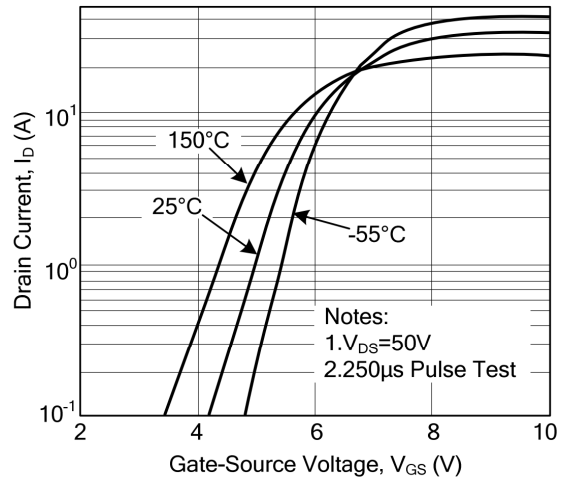
2. Transfer Characteristics
