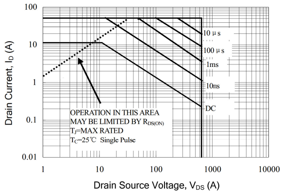
3. Maximum Safe Operating Area
